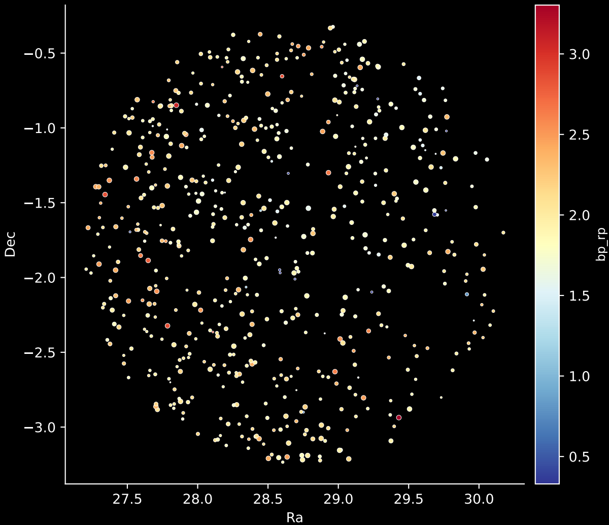
APOGEE DR17 Field: [034-06] Stars: 597
