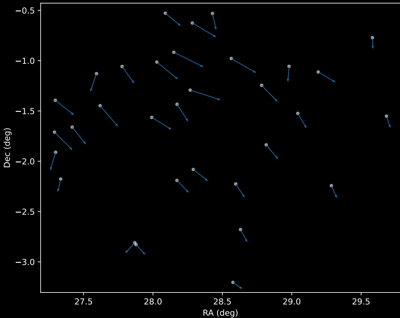
APOGEE DR17 Cluster 0 Proper Motion Vectors (n=32)
