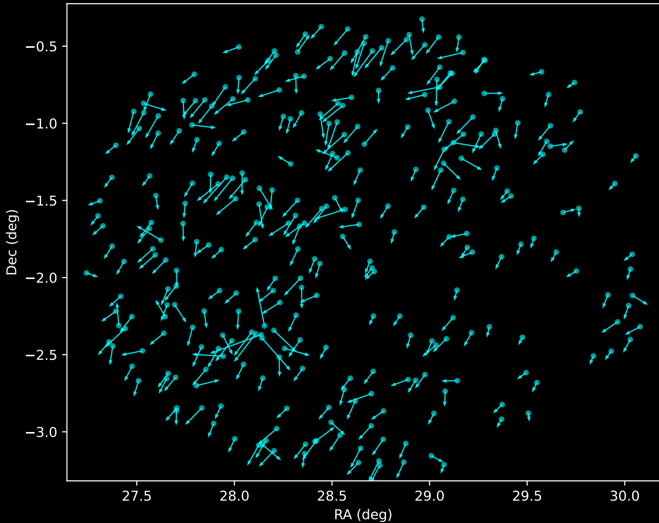
APOGEE DR17 Noise Stream Proper Motion Vectors (n=295)
