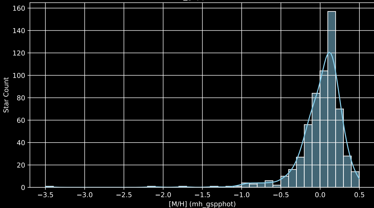
APOGEE DR17 Field: [034-06 [M/H] (mh_gspphot) (n= 591)
