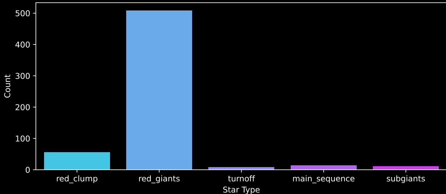
APOGEE DR17 Field: [034-06] Count plot of Star Type
