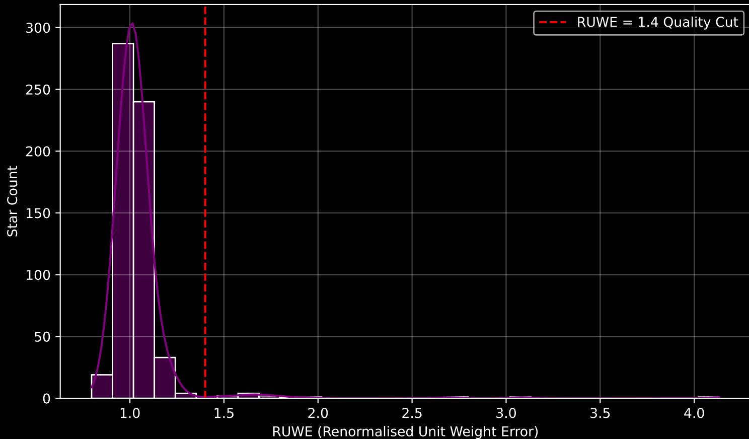
GAPOGEE DR17 Field [034-06] RUWE Distribution (n= 596)
