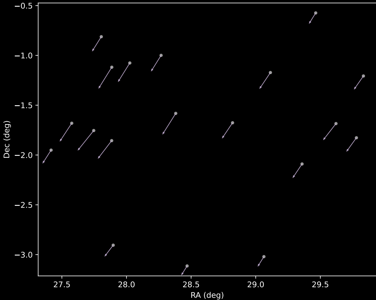
APOGEE DR17 Cluster 29 Proper Motion Vectors (n=19)
