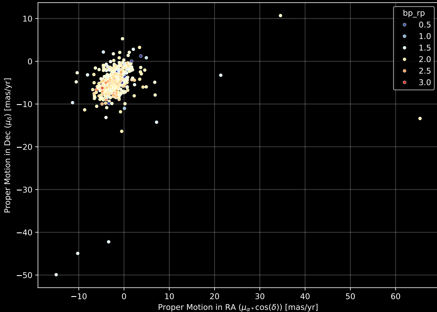
APOGEE DR17 Field: [034-06] Proper Motion Diagram (n= 597)
