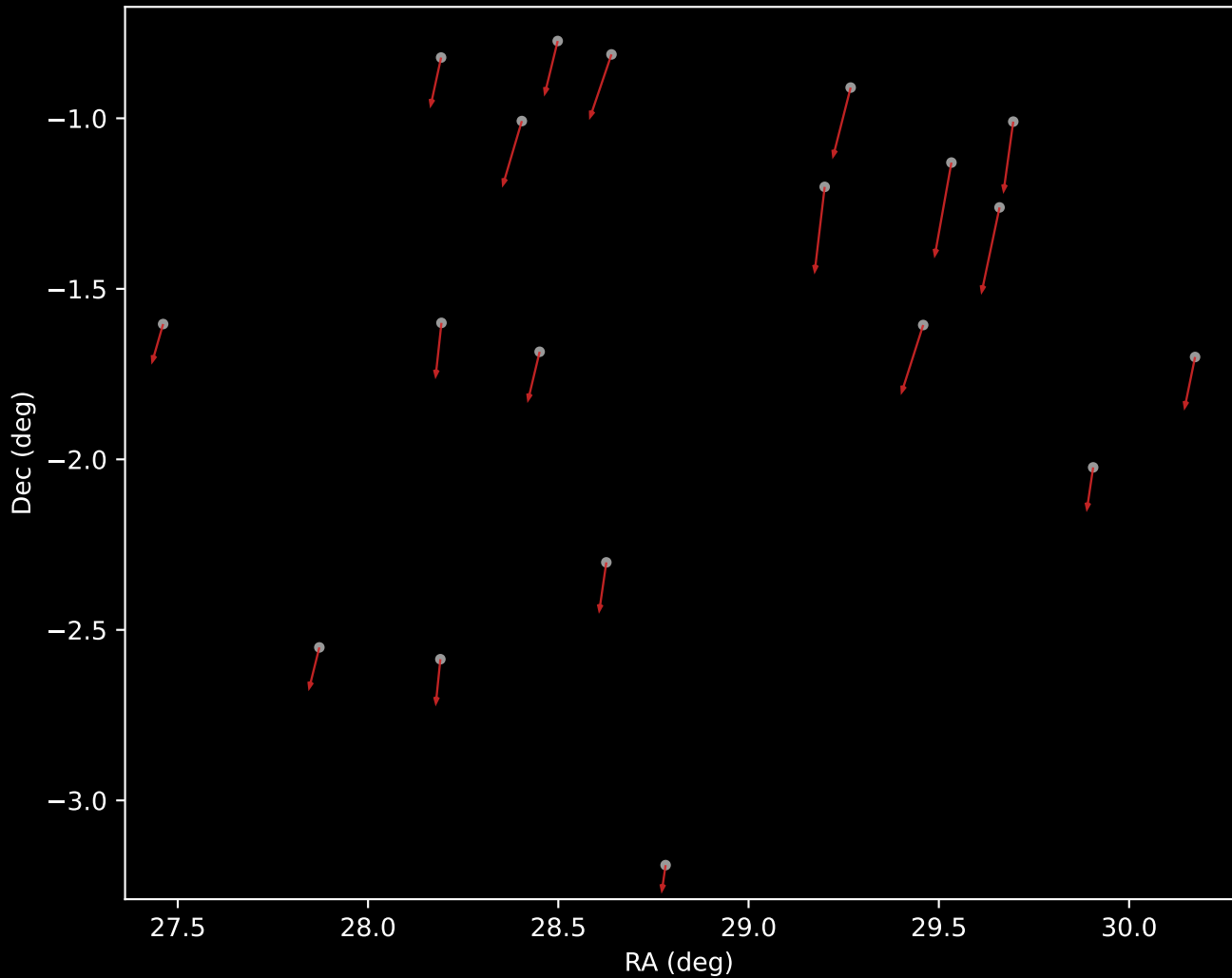
APOGEE DR17 Cluster 6 Proper Motion Vectors (n=19)
