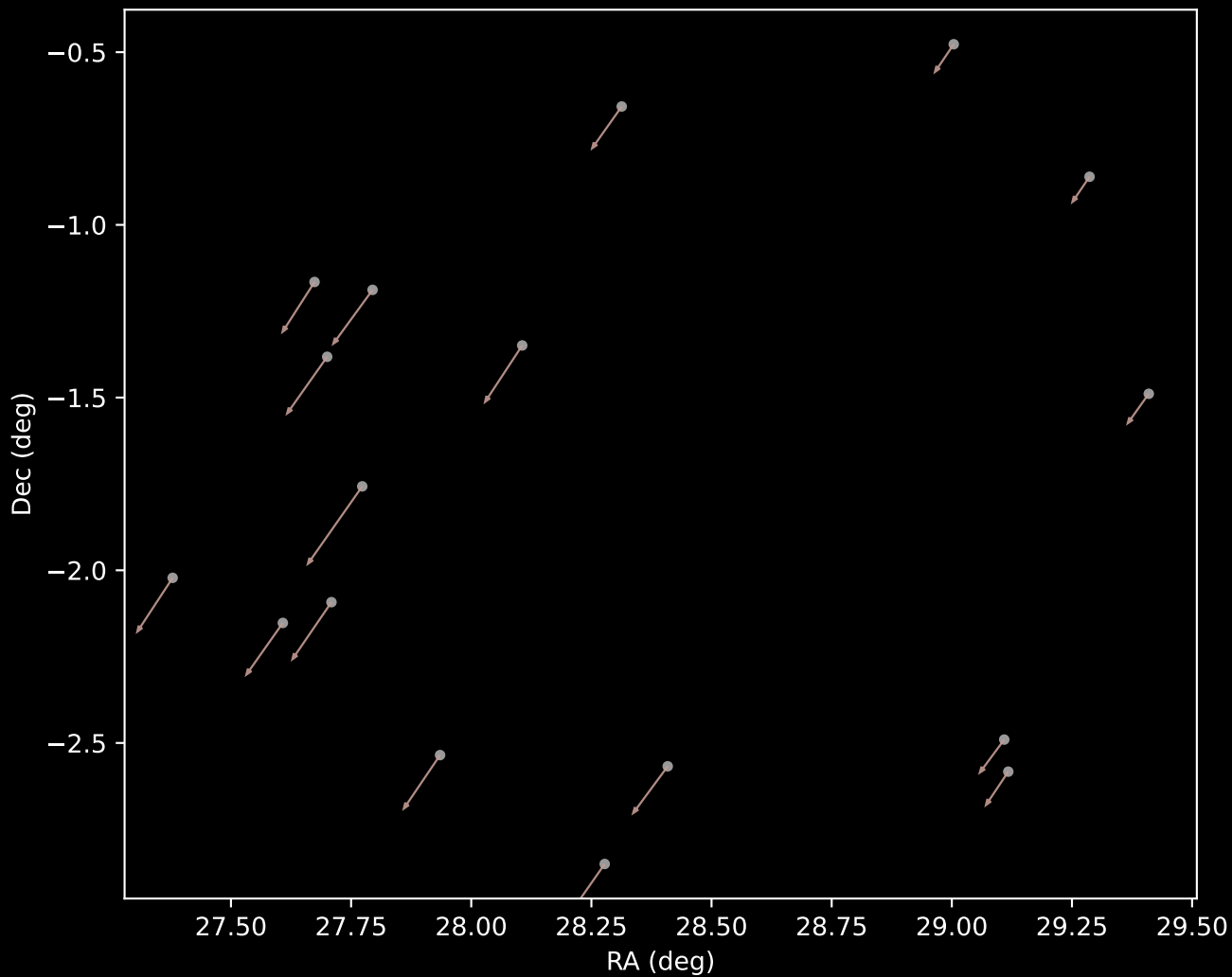
APOGEE DR17 Cluster 31 Proper Motion Vectors (n=17)
