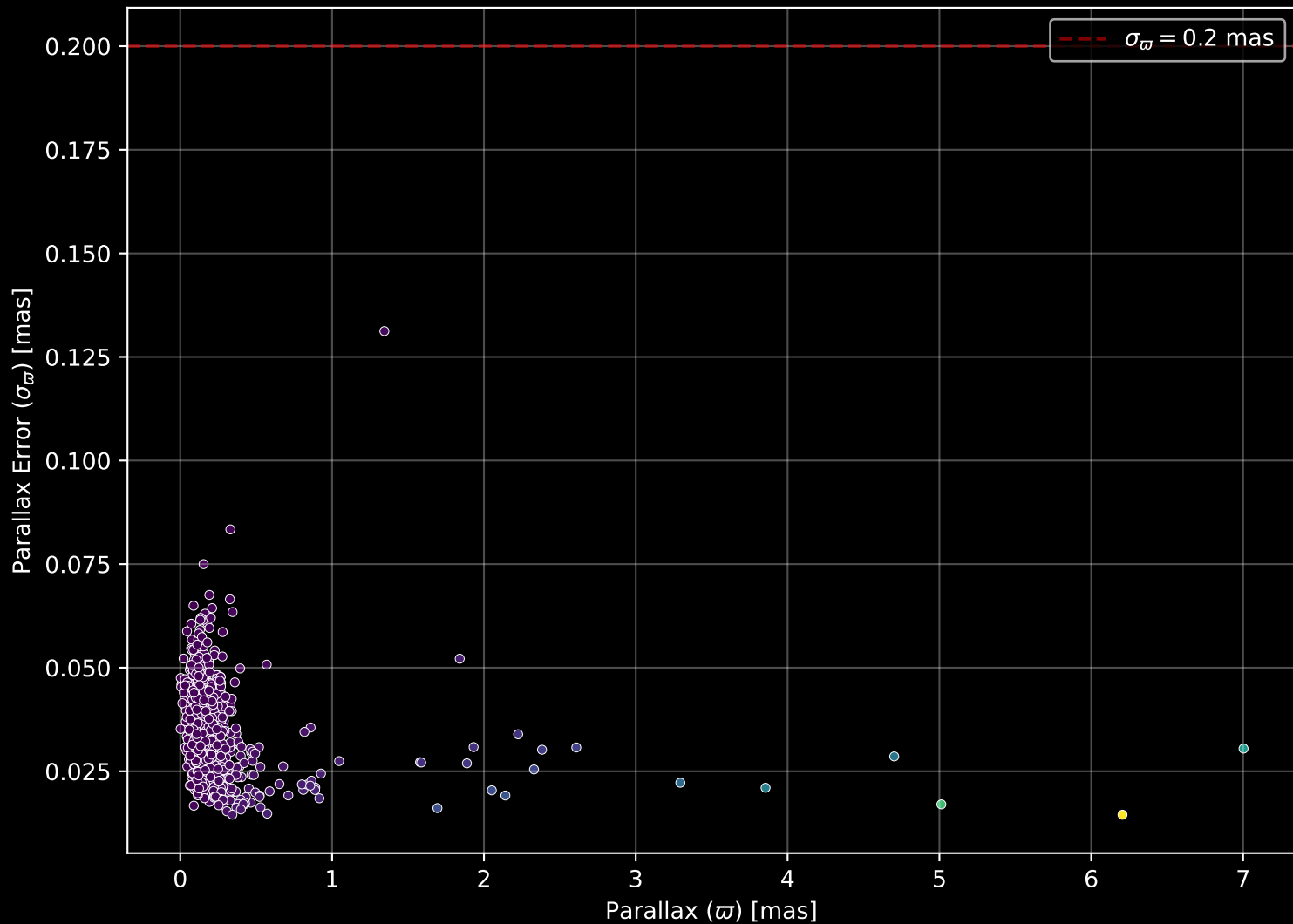
APOGEE DR17 Field: [034-06] Parallax Quality (n= 597)
