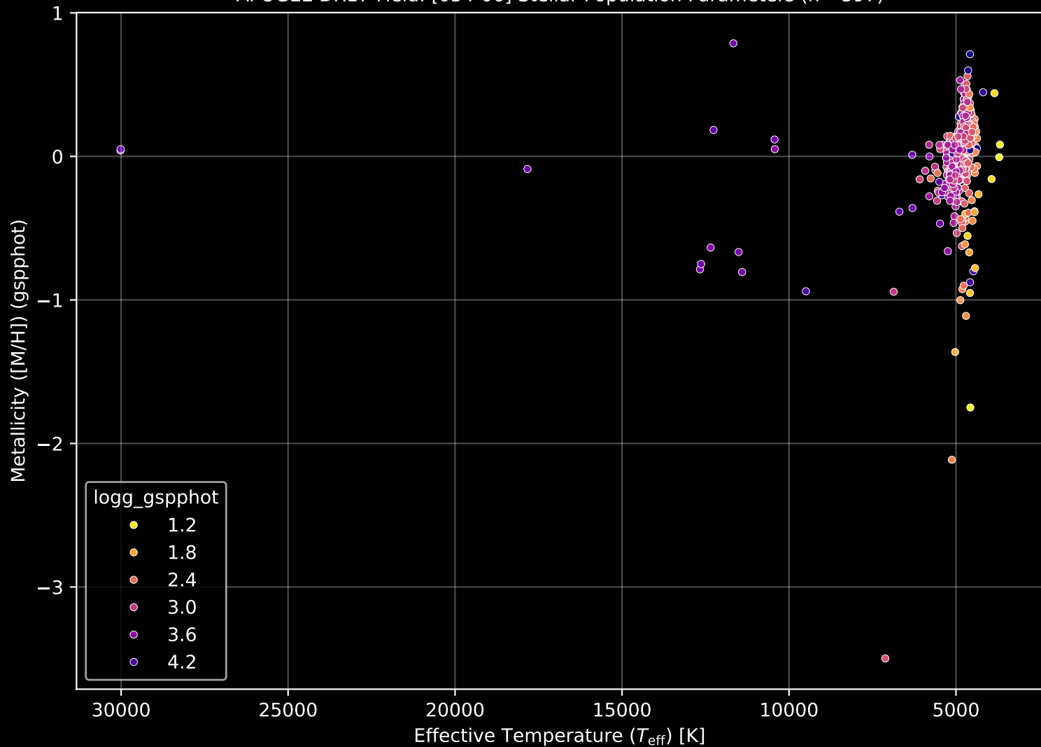
APOGEE DR17 Field: [034-06] Stellar Population Parameters (n= 597)
