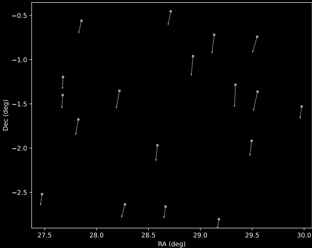
APOGEE DR17 Cluster 11 Proper Motion Vectors (n=18)
